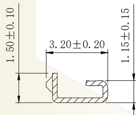
SEC C-C
