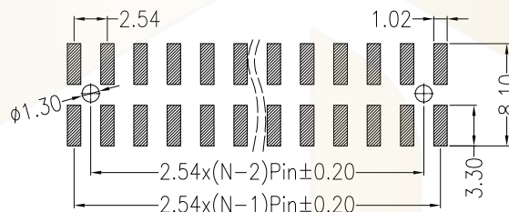
Recommended P.C.B Layout(Top Side) (PCB BOARD TOLERANCE±0.05)
