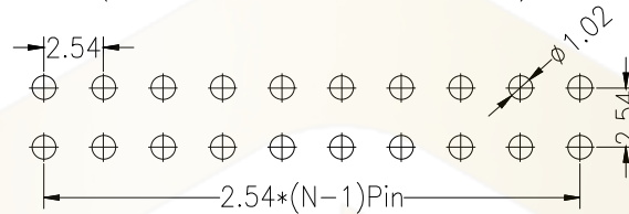
Recommended P.C.B Layout(Top Side) (PCB BOARD TOLERANCE±0.05)
