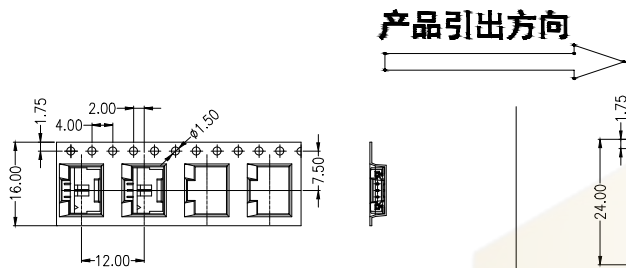
02~03 CONTACTS
