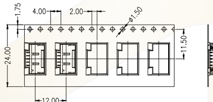
4~7 CONTACTS
