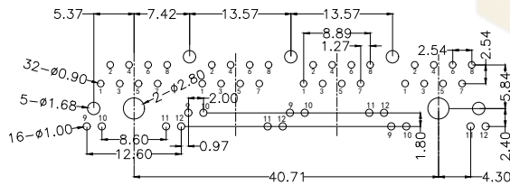
RECOMMENDED PCB LAYOUT VIEWED FROM COMPONENT SIDE
