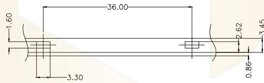
RECOMMENDED BRACKET CUTOUT
