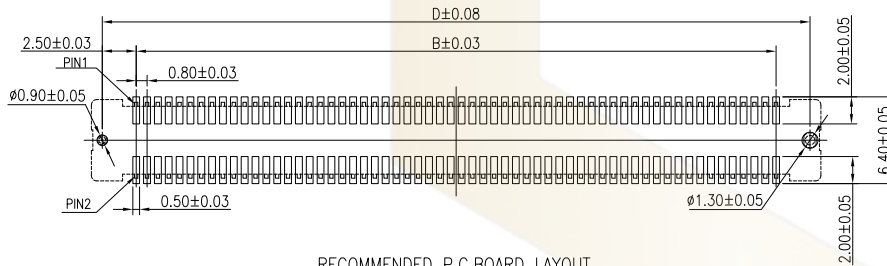
RECOMMENDED P.C.B. BOARD LAYOUT
